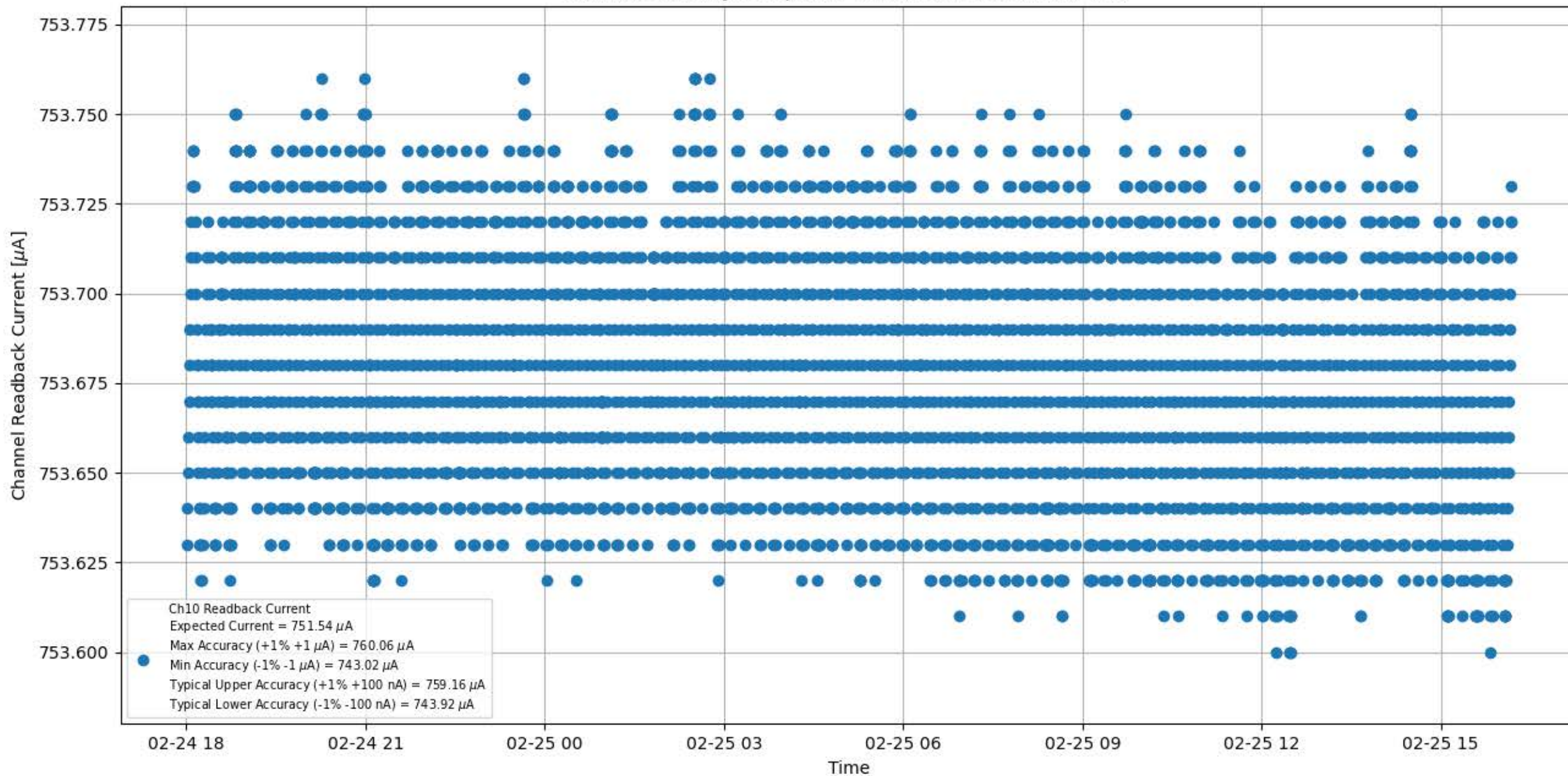
Current Stability 750 \mu\text{A} for Module #094 Channel #10
