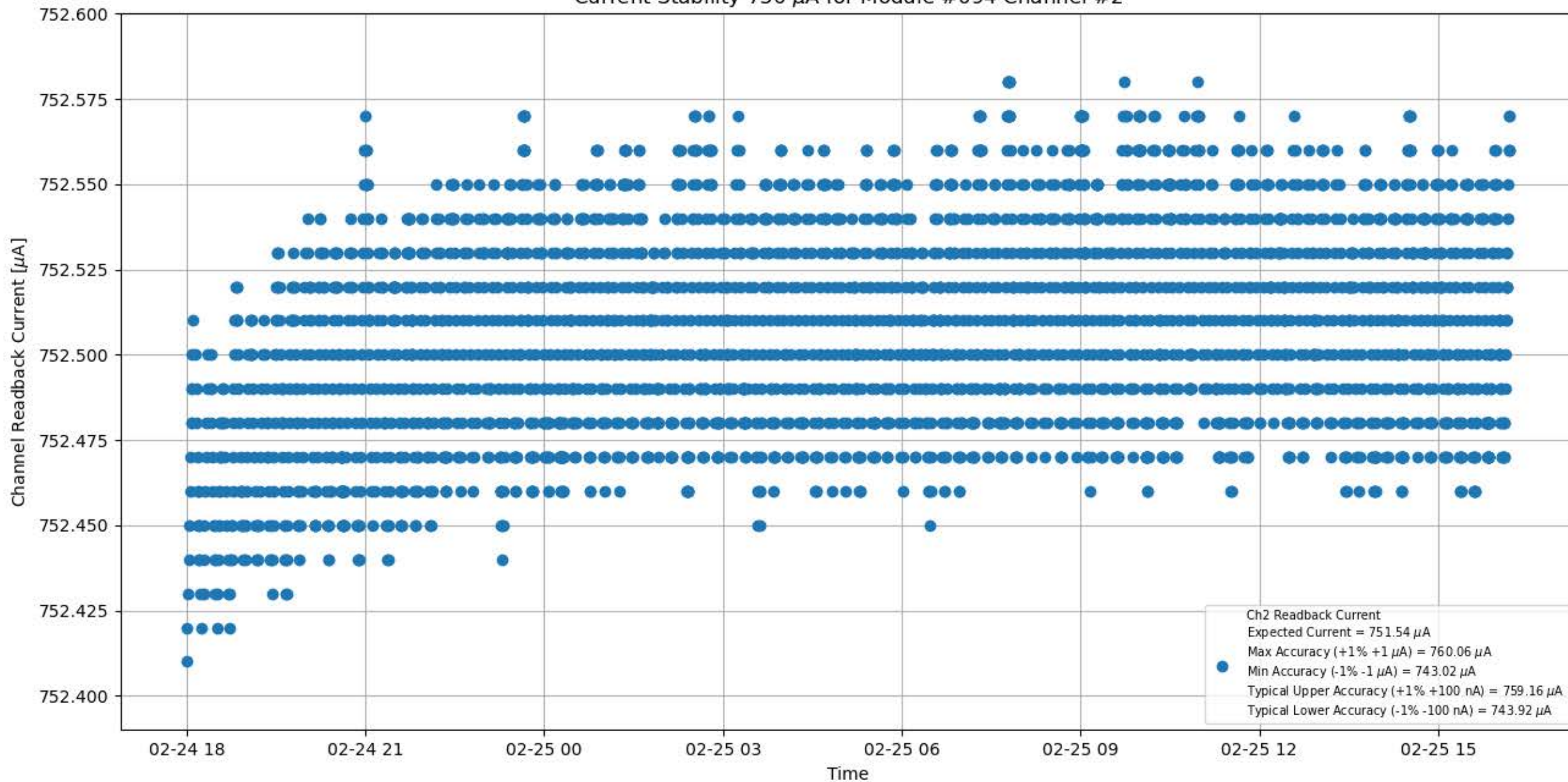
Current Stability 750 \mu\text{A} for Module #094 Channel #2
