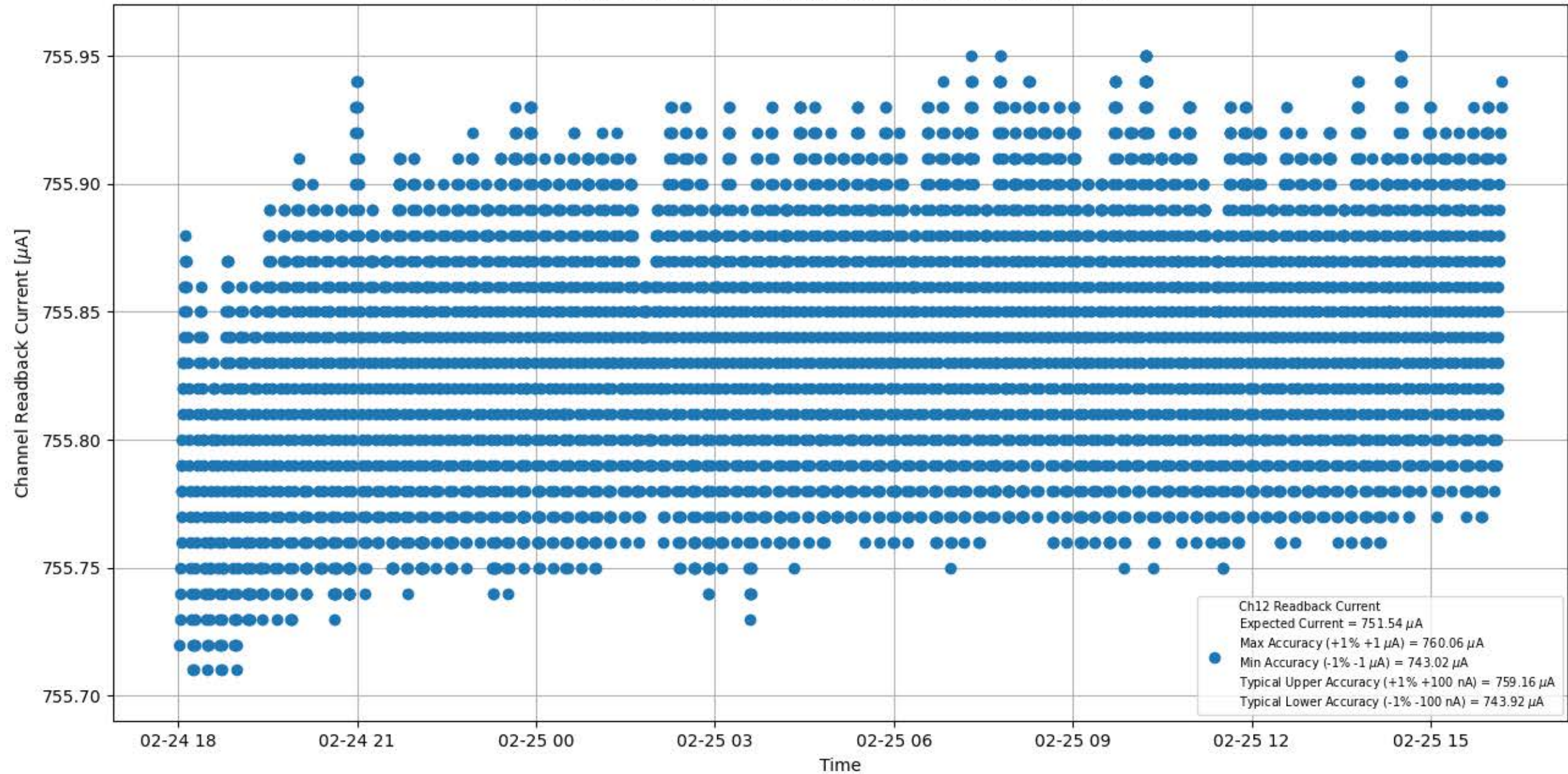
Current Stability 750 \mu A for Module #094 Channel #12
