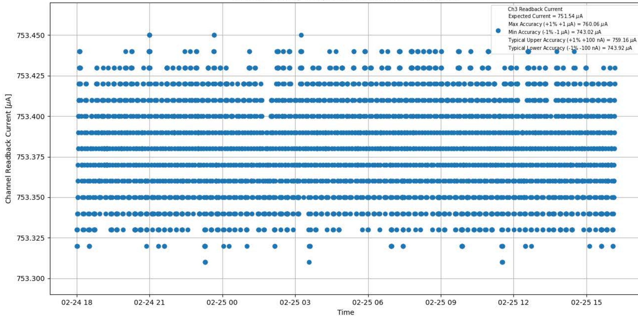
Current Stability 750 \mu\text{A} for Module #094 Channel #3
