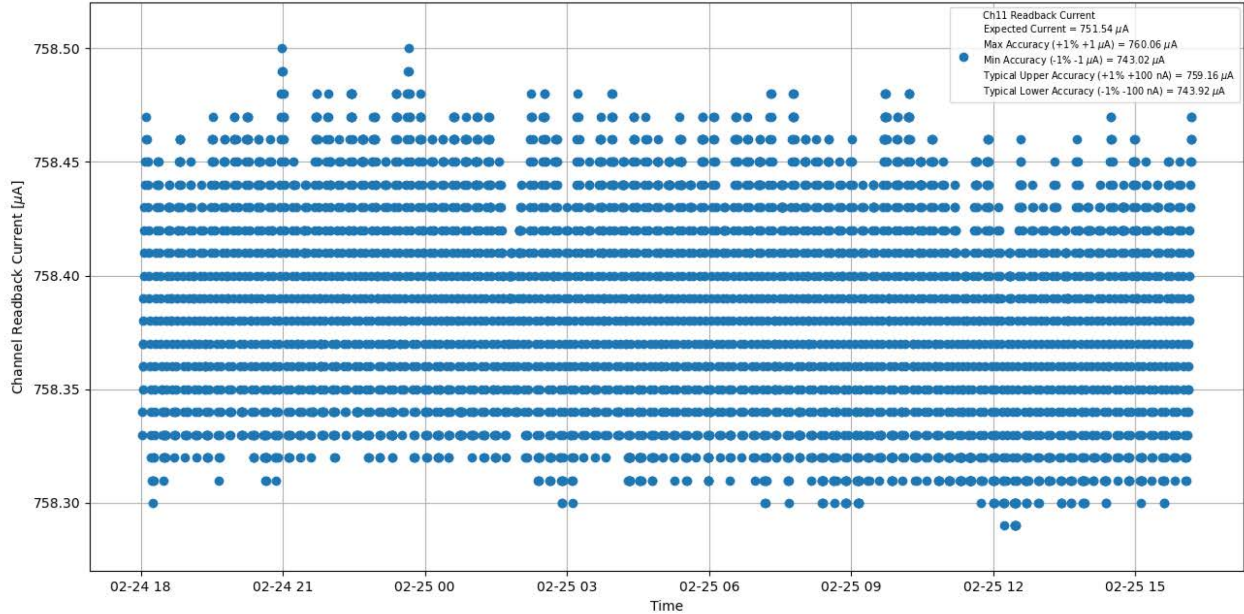
Current Stability 750 \mu\text{A} for Module #094 Channel #11
