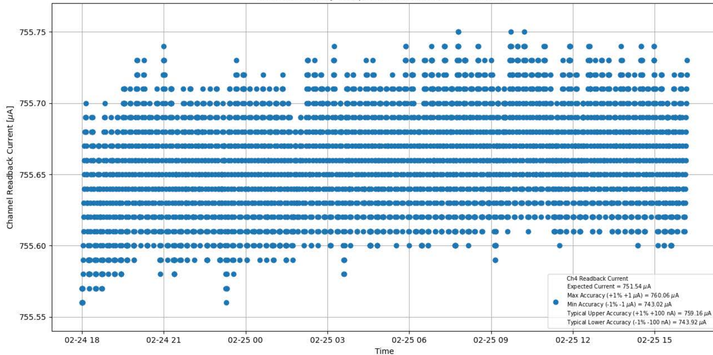
Current Stability 750 \mu\text{A} for Module #094 Channel #4
