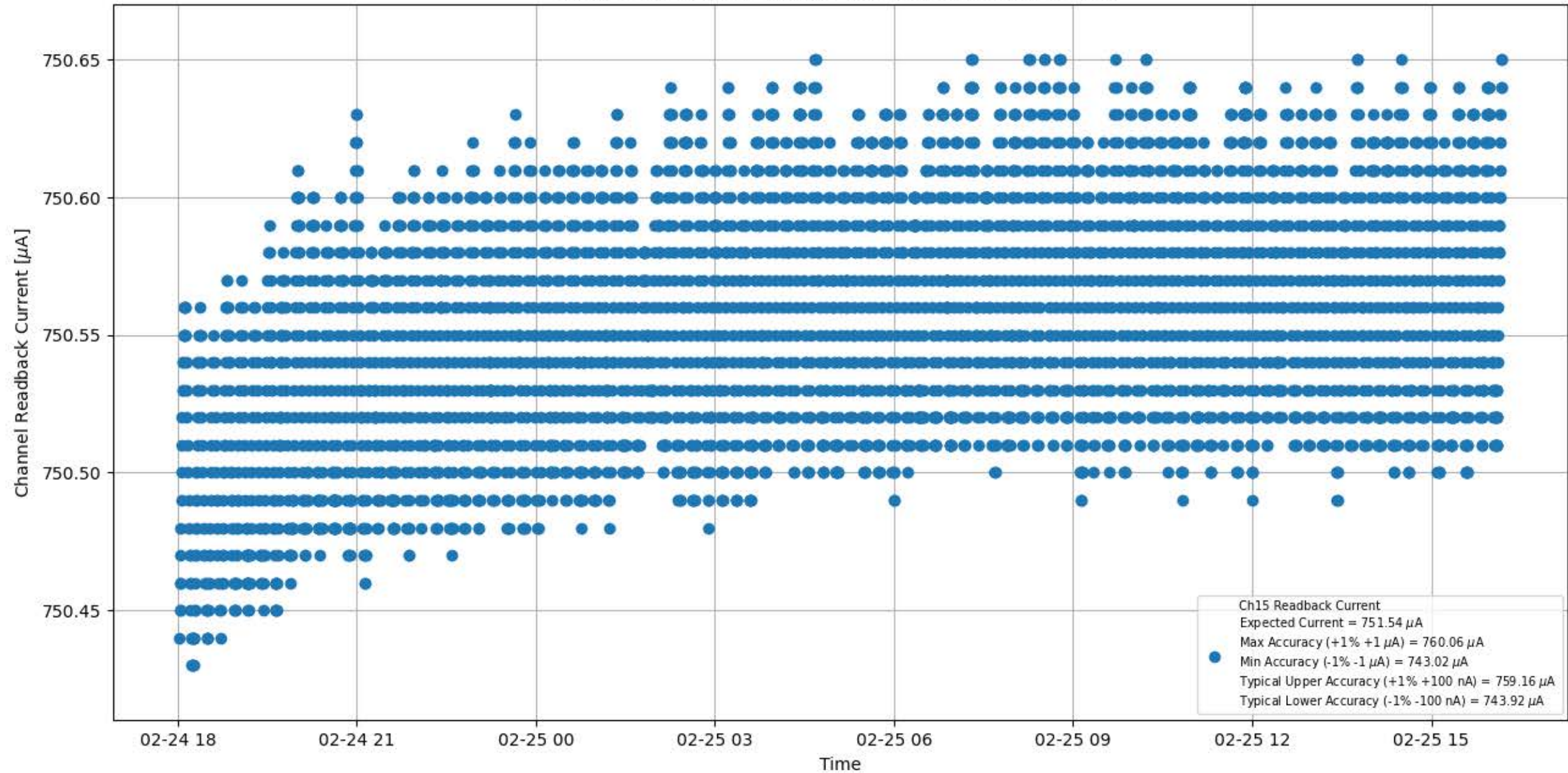
Current Stability 750 \mu A for Module #094 Channel #15
