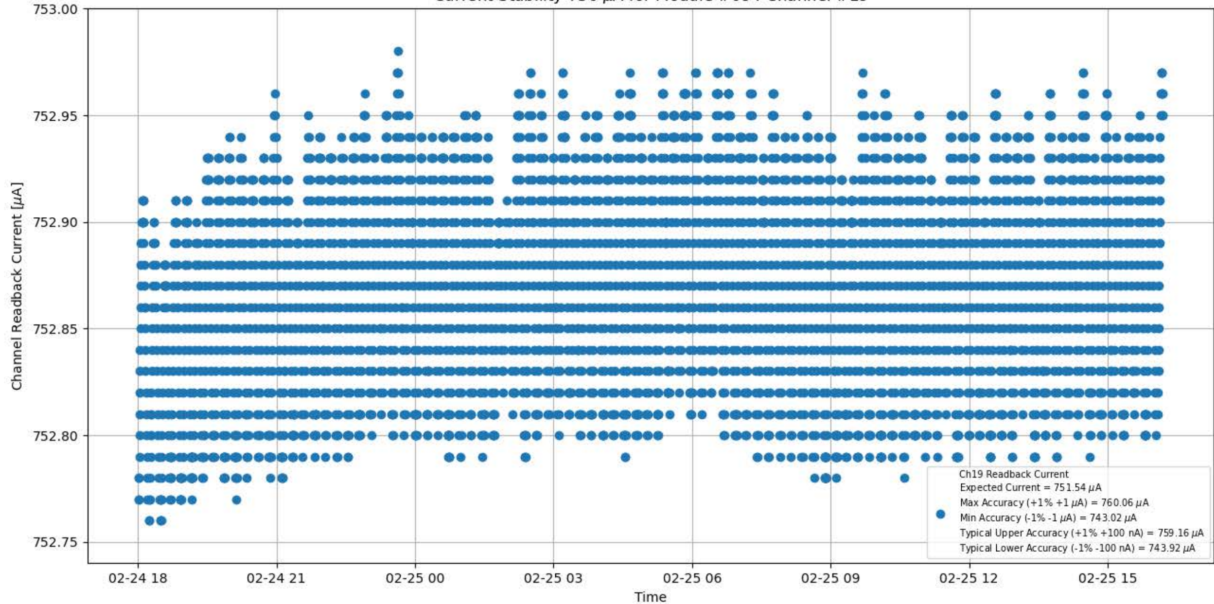
Current Stability 750 \mu A for Module #094 Channel #19
