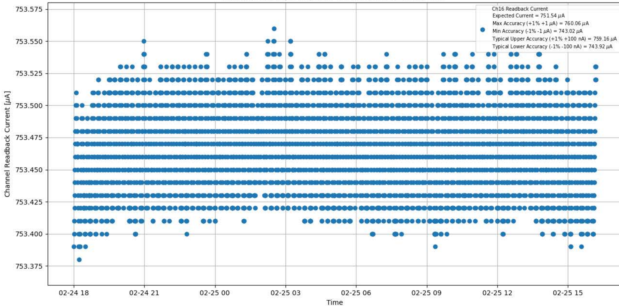
Current Stability 750 \mu A for Module #094 Channel #16
