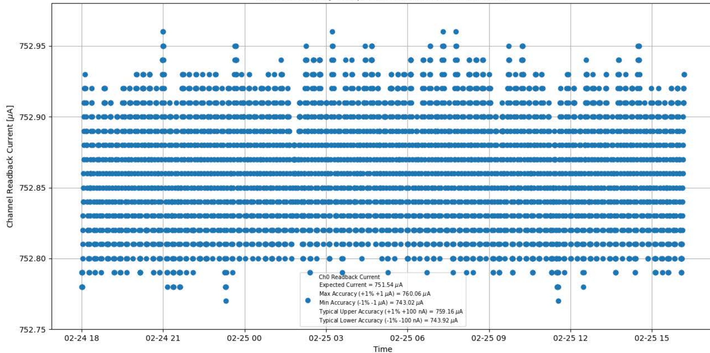
Current Stability 750 \mu A for Module #094 Channel #0
