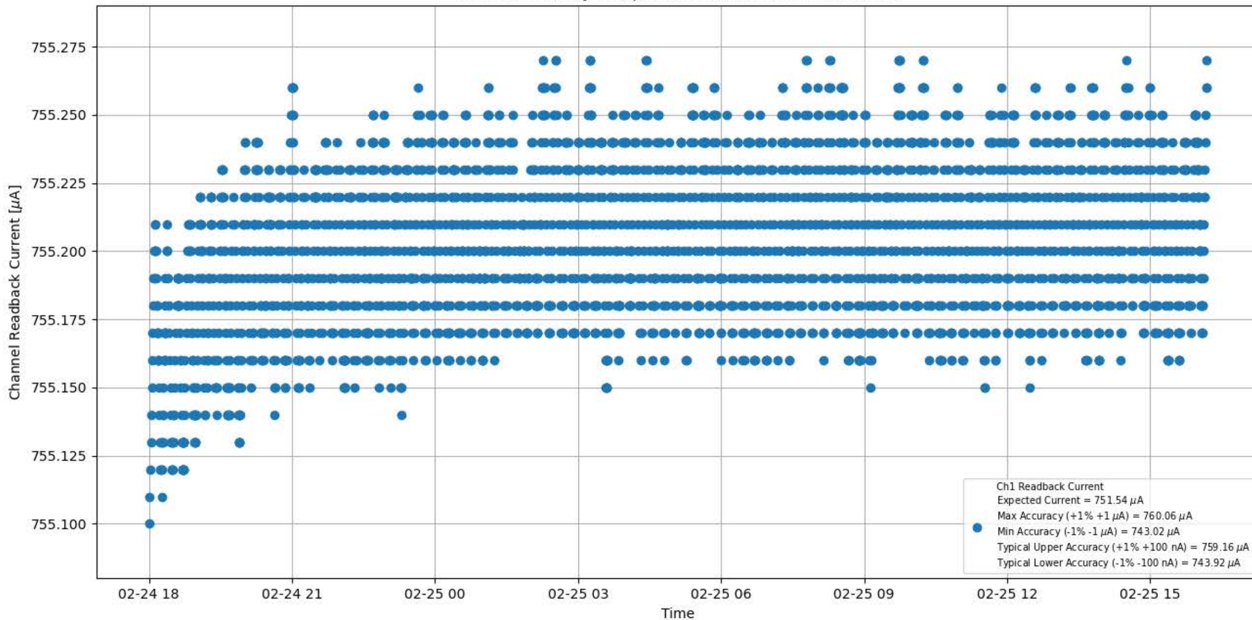
Current Stability 750 \mu\text{A} for Module #094 Channel #1
