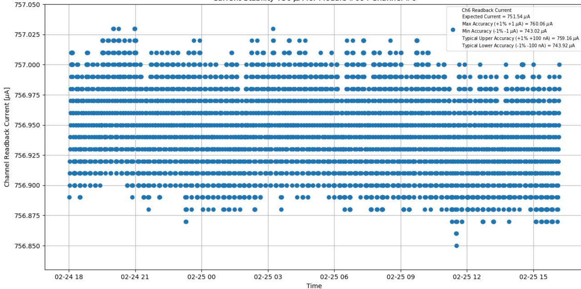
Current Stability 750 \mu\text{A} for Module #094 Channel #6
