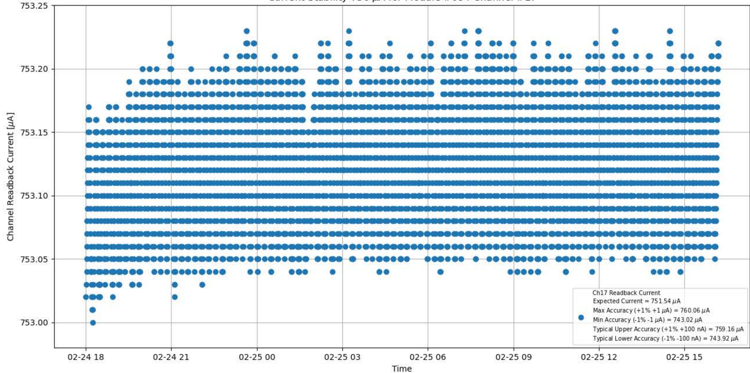
Current Stability 750 \mu A for Module #094 Channel #17
