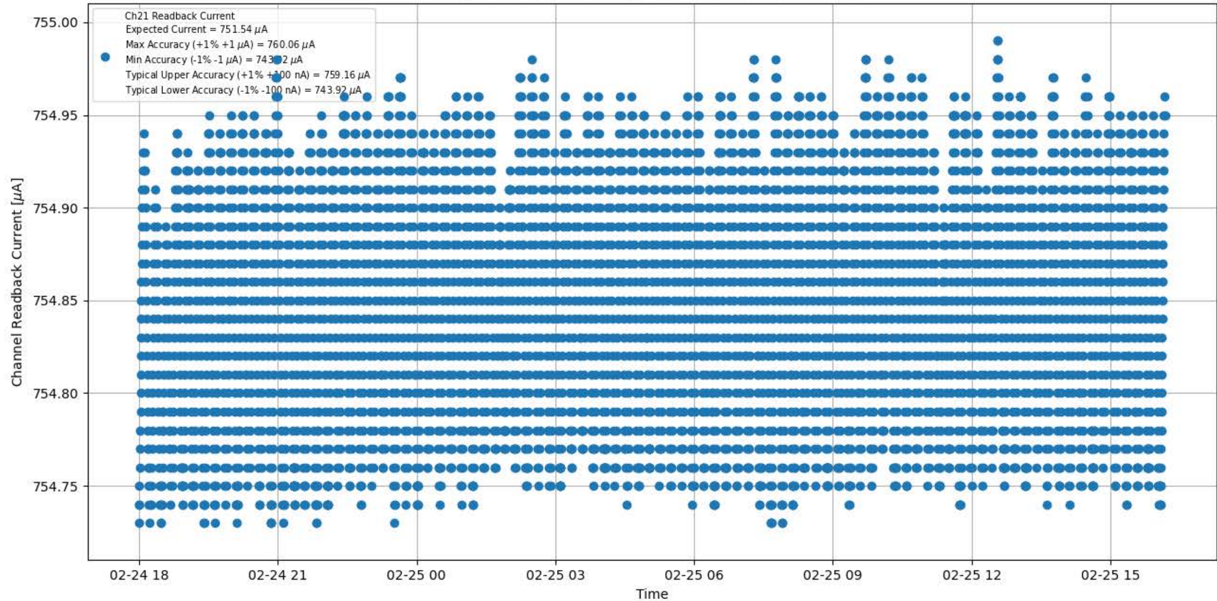
Current Stability 750 \mu A for Module #094 Channel #21
