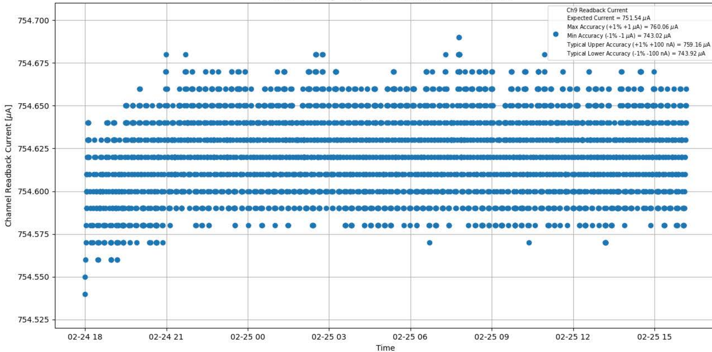
Current Stability 750 \mu\text{A} for Module #094 Channel #9
