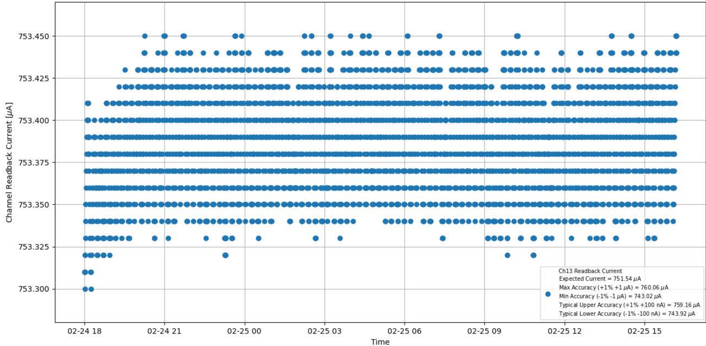
Current Stability 750 \mu A for Module #094 Channel #13
