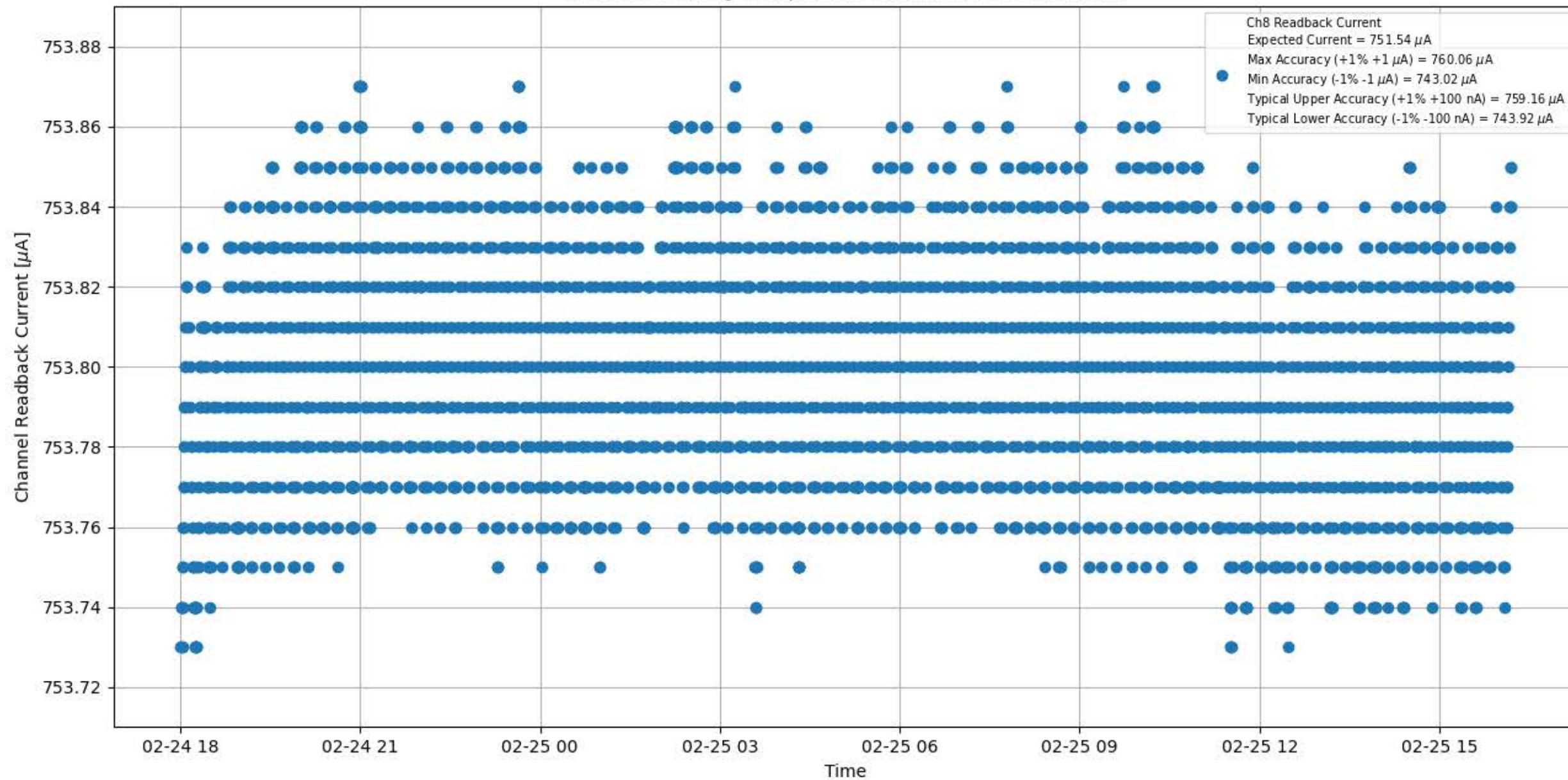
Current Stability 750 \mu\text{A} for Module #094 Channel #8
