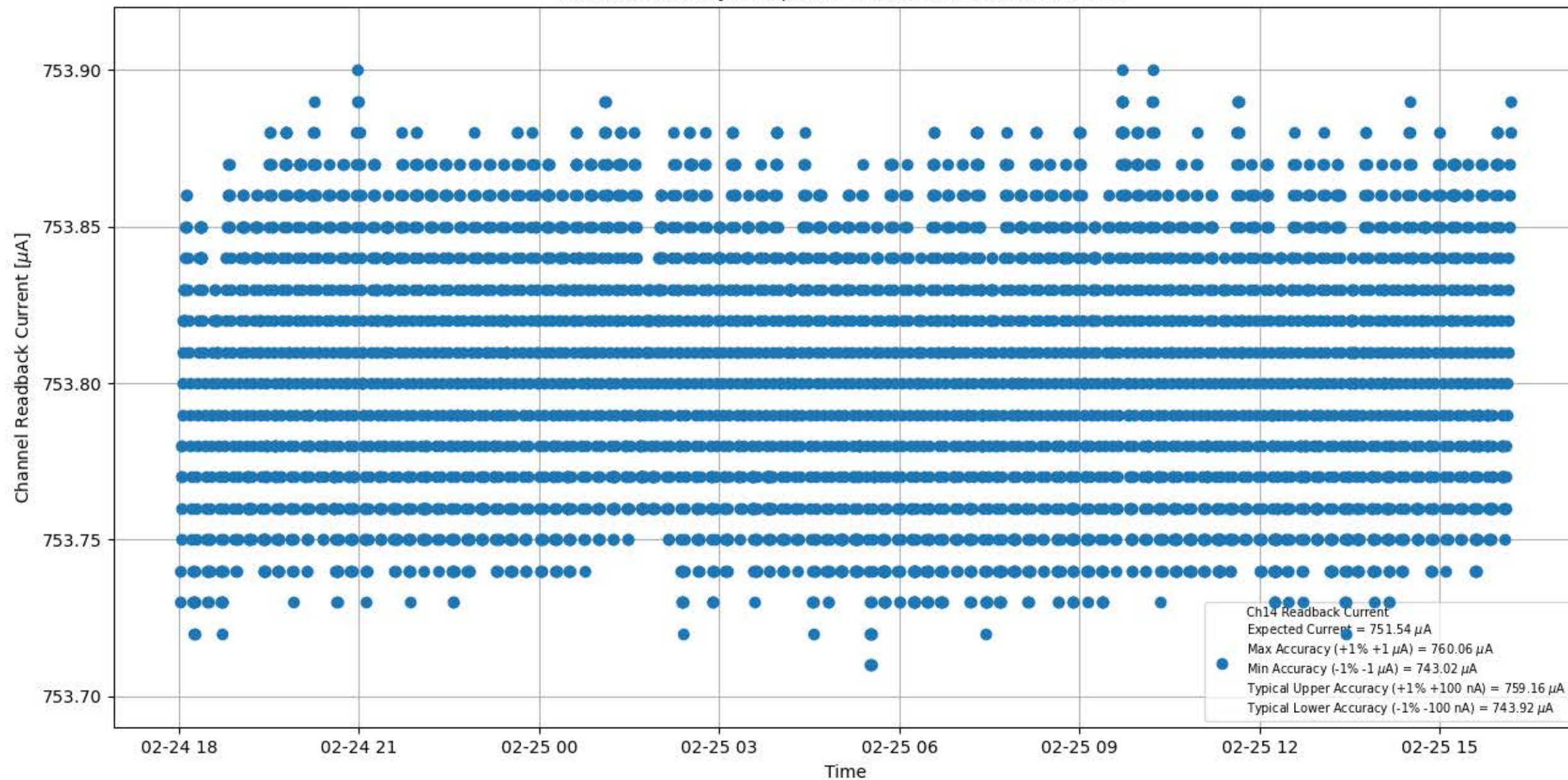
Current Stability 750 \mu A for Module #094 Channel #14
