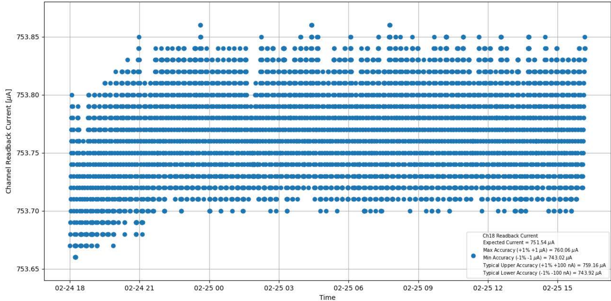
Current Stability 750 \mu A for Module #094 Channel #18
