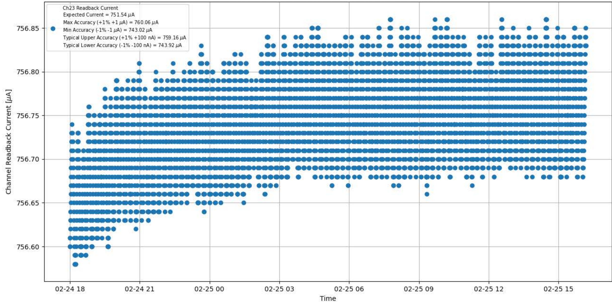
Current Stability 750 \mu\text{A} for Module #094 Channel #23
