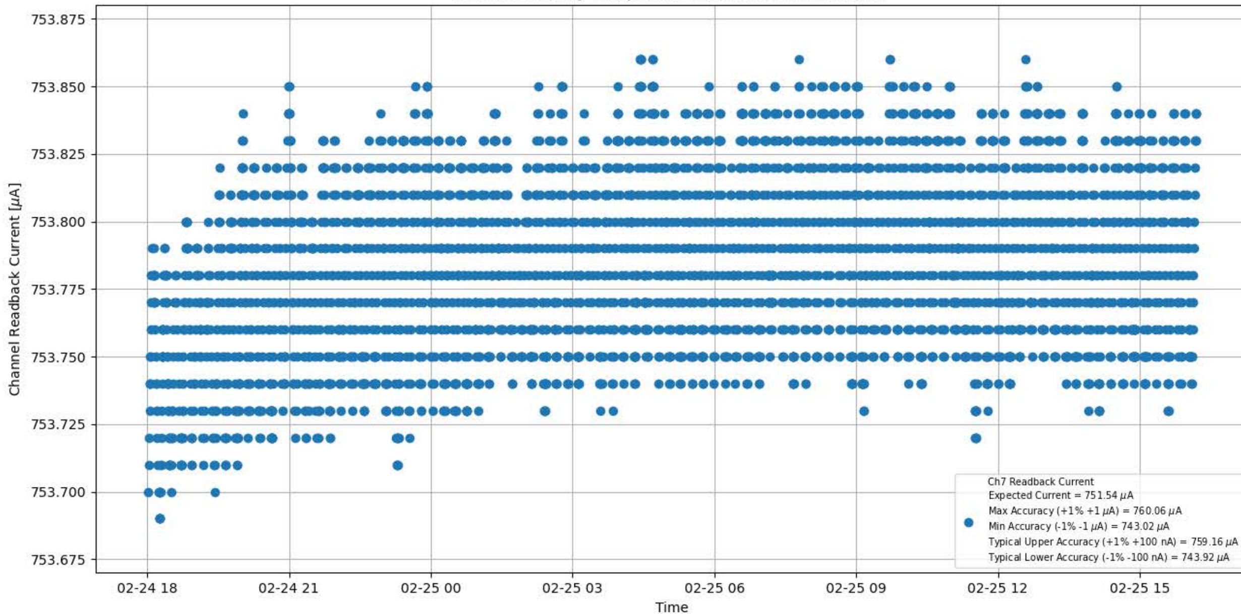
Current Stability 750 \mu\text{A} for Module #094 Channel #7
