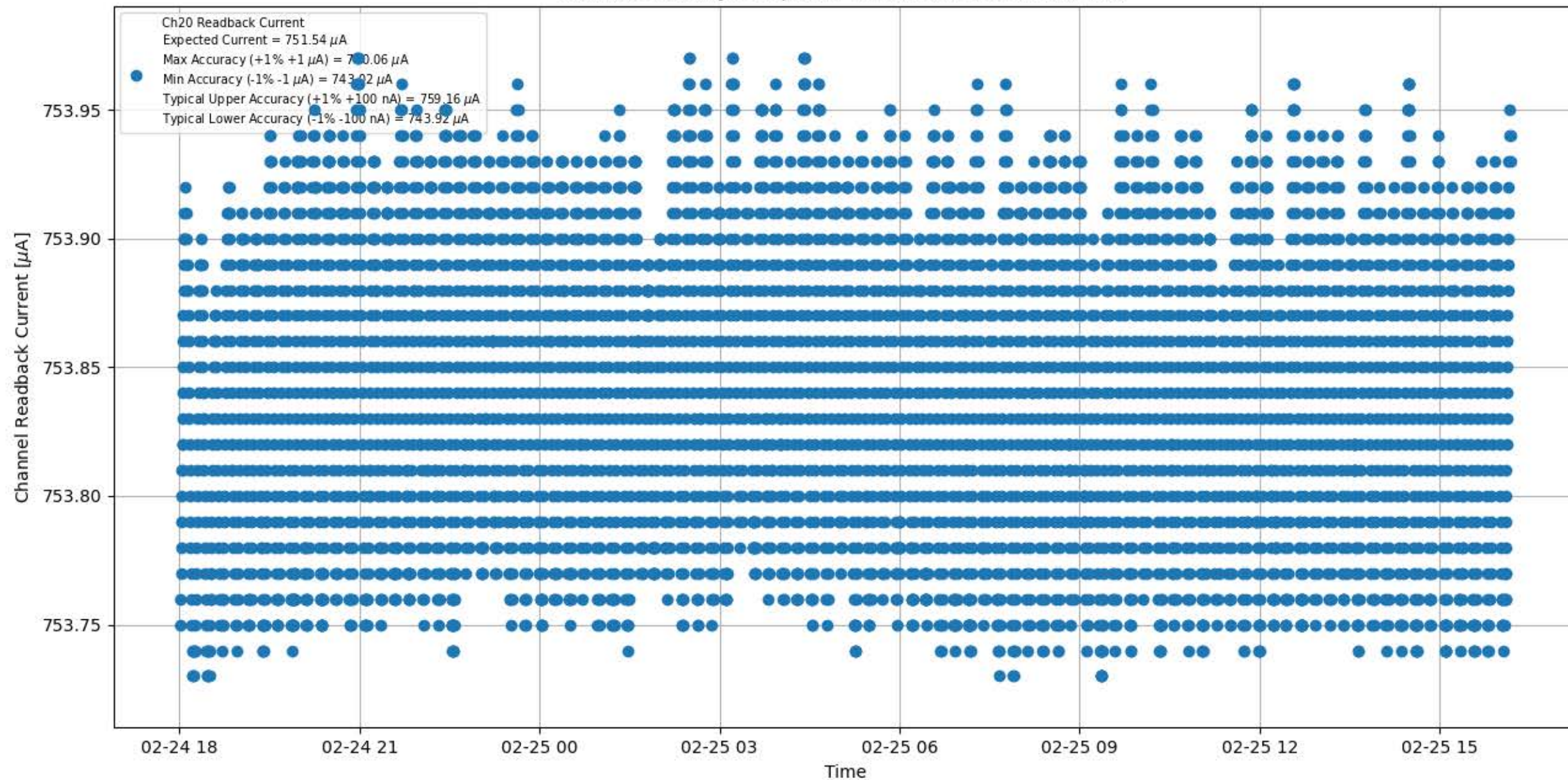
Current Stability 750 \mu\text{A} for Module #094 Channel #20
