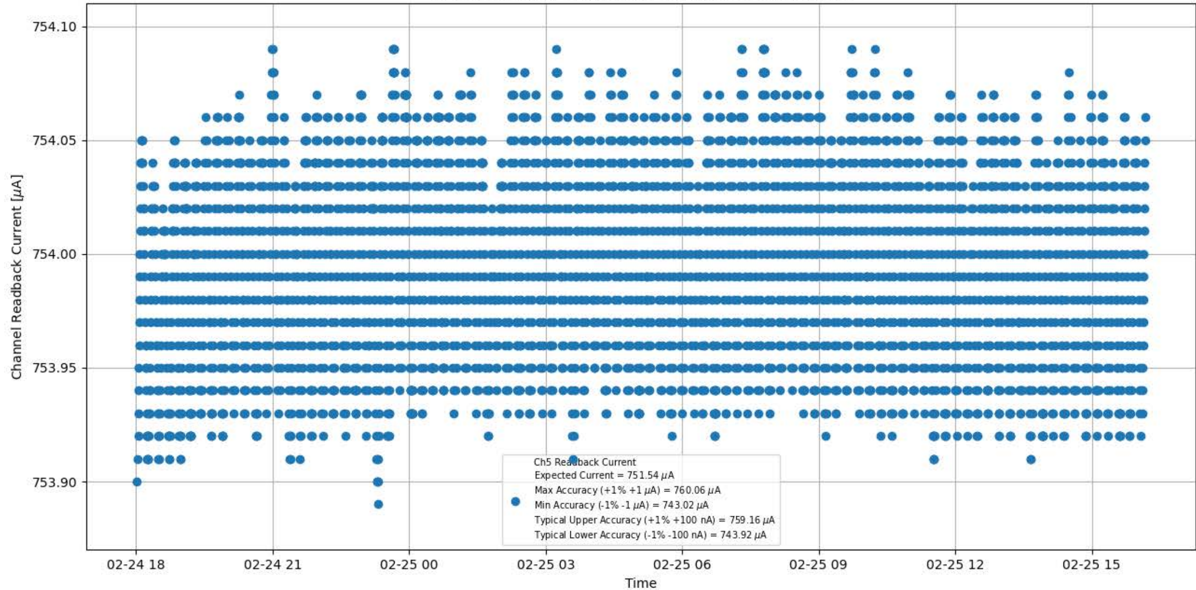
Current Stability 750 \mu A for Module #094 Channel #5
