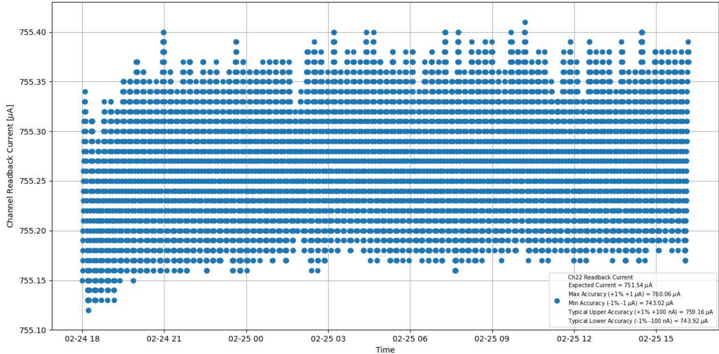
Current Stability 750 \mu\text{A} for Module #094 Channel #22
